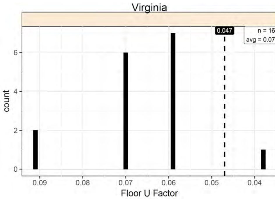
Figure 3.16. Floor U-Factors
