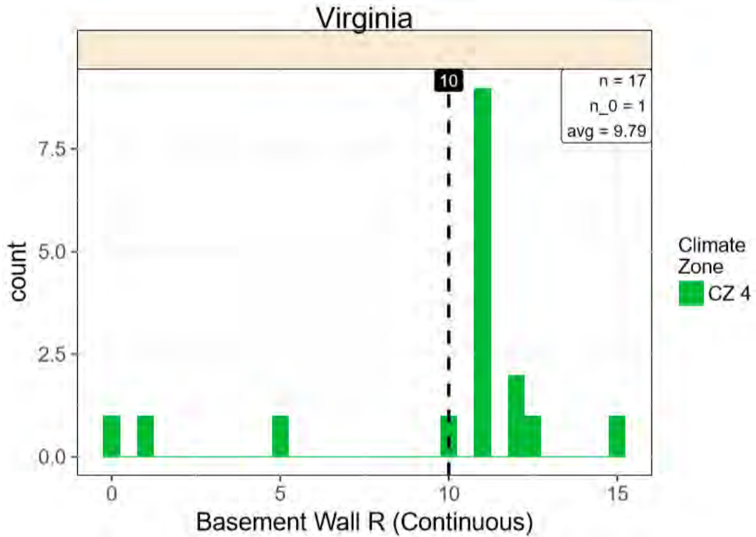
Figure 3.12. Basement Wall Continuous R-Values
