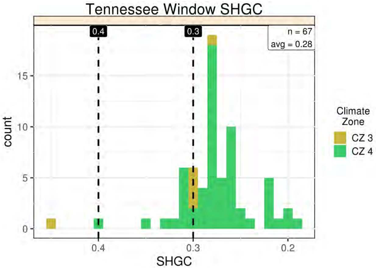
Figure 3.2. Window SHGC for Tennessee
